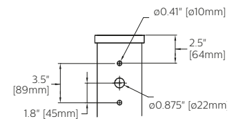
Drill template
