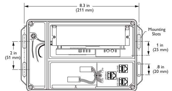
Mounting Dimensions
