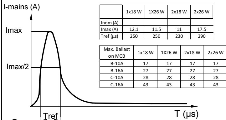
Ballast HF-H
