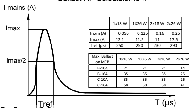
Ballast HF-Selectalume II
