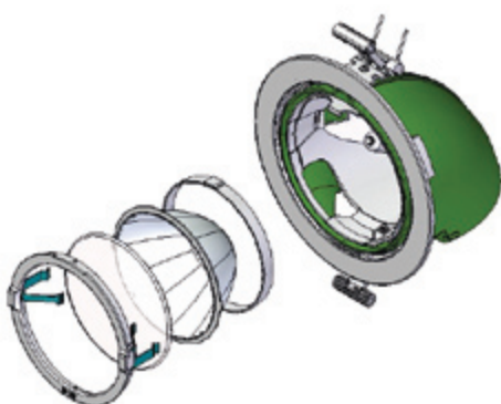
Exploded view of the 24° Elbow version
