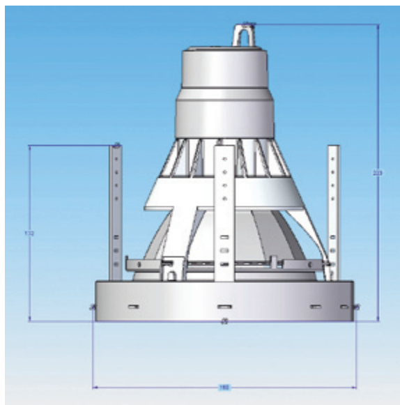
Dimensions of the ceiling rim
