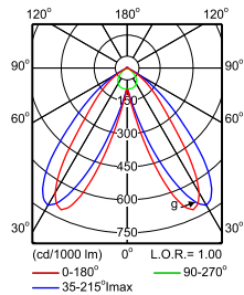
IFPS_4MX400 581 1xLED40S/830 PSD DA- Polar Normal (separate)
