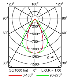
IFPS_4MX400 G3 581 1xLED55S/840 PSD NB- Polar Normal (separate)
