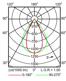
IFPS_4MX400 G3 581 1xLED66S/830 PSD NB- Polar Normal (separate)
