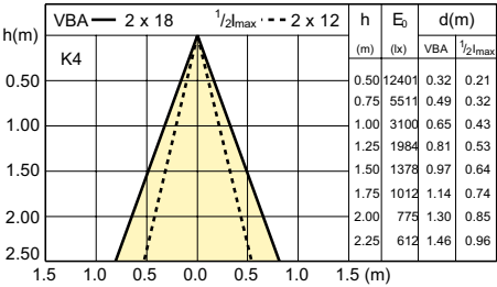
LDBE_HDICHRO_35W_24D-Beam diagram
