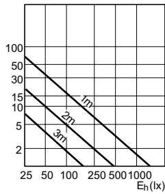
LDAC_HPAR30S_75W_30D-Accent diagram
