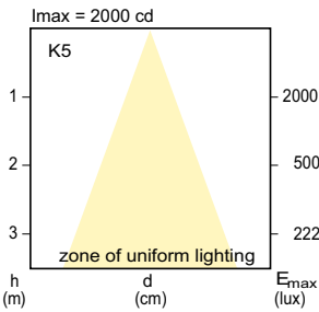
LDBE_HPAR30S_75W_30D-Beam diagram
