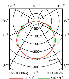
IFPS_TMS022 2xTL-D18W +GMS022 R-Polar Normal (separate)
