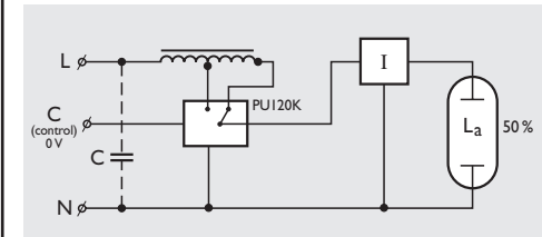
Power Switch PU120K, dimming 50%
