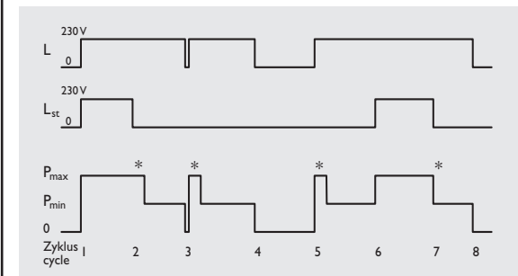
Power Switch PU120K, no dimming
