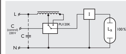
Power Switch PU120K, no dimming
