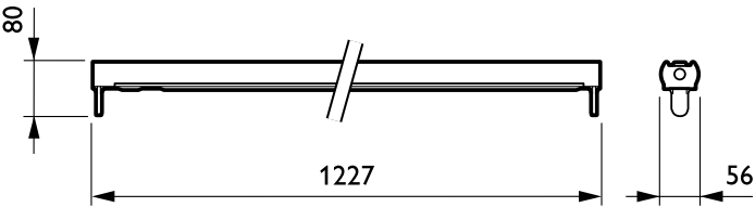
Dimensional drawing
