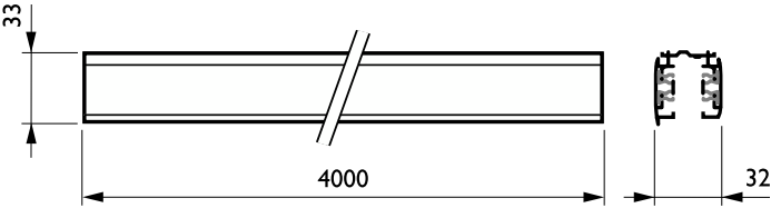
Dimensional drawing
