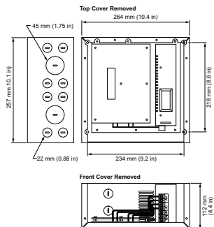
Power/data supply units ZCX400
