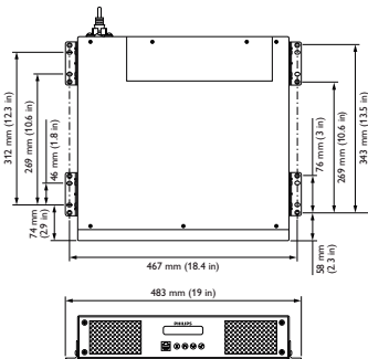
Power/data supply units ZCX200
