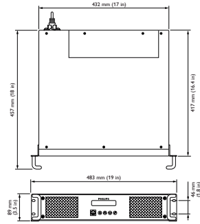
Power/data supply units ZCX400
