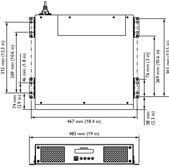
Power/data supply units ZCX400
