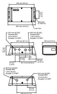
Power/data supply units ZCX400
