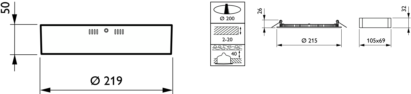
Dimensional drawing
