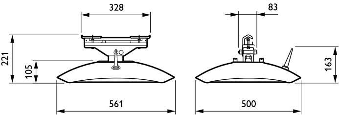
Dimensional drawing
