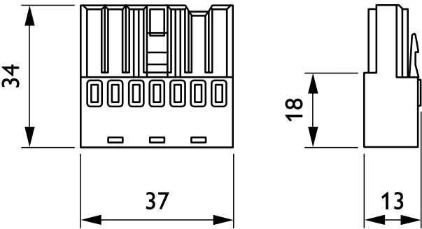
Dimensional drawing
