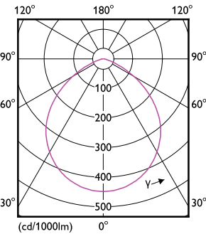
Light Distribution Diagram - DN060B LED85/840 PSU WH
