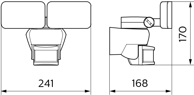
Dimensional drawing
