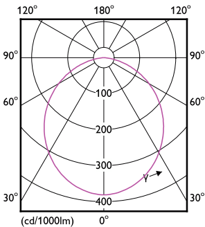
Light Distribution Diagram - DN027B LED3/CW D90 RD
