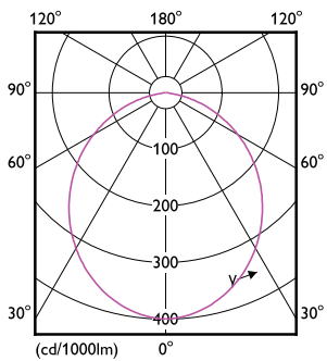
Downlight DN027B LED6 WW D100 RD
