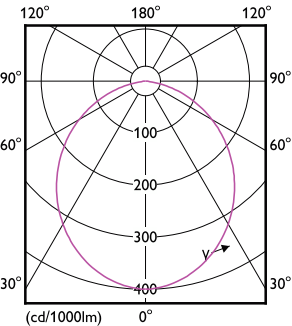
Light Distribution Diagram - DN027B LED6/WW D150 RD
