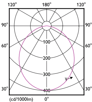
Light Distribution Diagram - DN027B LED9/WW D150 RD
