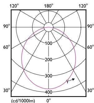
Light Distribution Diagram - DN027B LED12/NW D175 RD
