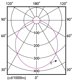
Light Distribution Diagram - DN027B LED15/WW D200 RD
