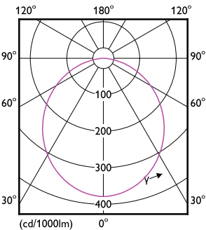
Light Distribution Diagram - DN027B LED15/NW D200 RD
