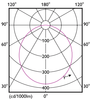
Light Distribution Diagram - DN027B LED20/WW D200 RD
