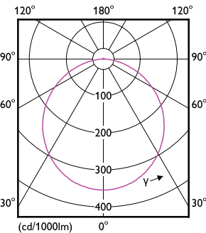
Light Distribution Diagram - DN027B LED3/WW L100 SQ
