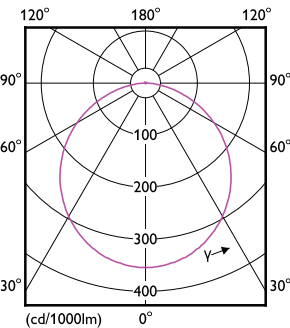
Light Distribution Diagram - DN027B LED3/CW L100 SQ
