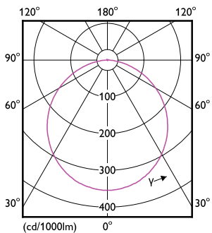
Light Distribution Diagram - DN027B LED3/CW L100 SQ
