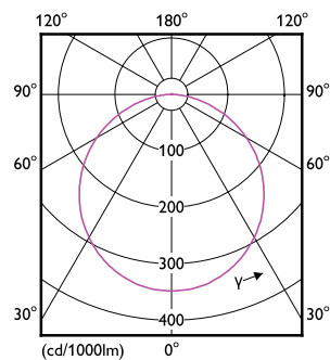
General uniform lighting - DN027B LED6/NW L125 SQ Light Distribution Diagram - DN027B LED6/NW L125 SQ
