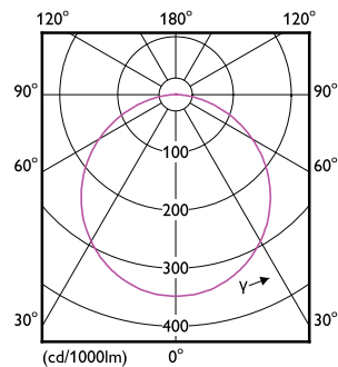
Light Distribution Diagram - DN027B LED6/CW L125 SQ
