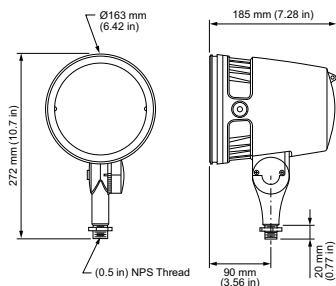
BCP462 G2 19xLED-HB/RGBW HMA GR
