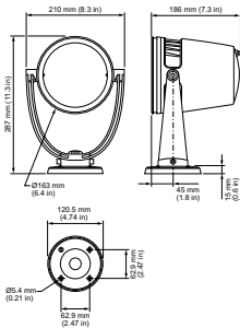
BCP462 G2 19xLED-HB/RGBW BK
