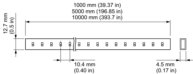
BGC452 4000 IP40 L10000 STRIP ONLY
