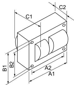
HPS BAL 400W S51 120/277/347V KIT
