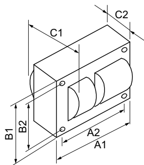
LPS BAL 18W L69 120/277V C&C
