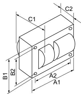
HPS BAL 250W S50 120/208/240V C&C
