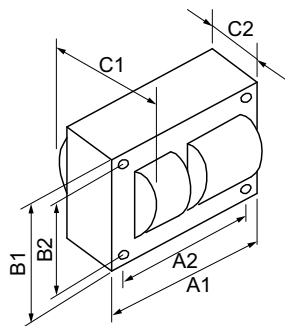
HPS BAL 200W S66 QUAD KIT
