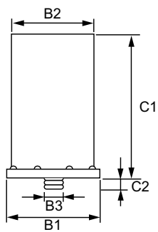
MH BAL 400W M59 QUAD WP
