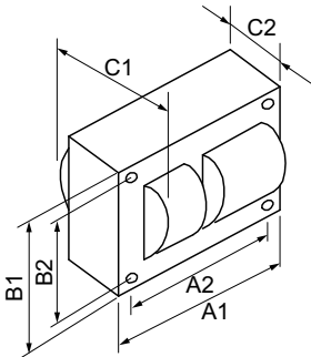
MH BAL 50W M110 QUAD KIT
