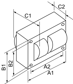
HPS BAL 400W S51 230/400/480V C&C
