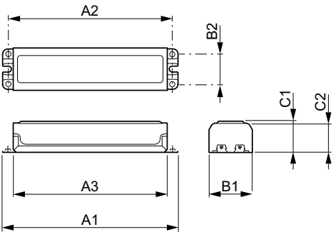
100W/4.1A-24V INTELLIVOLT
