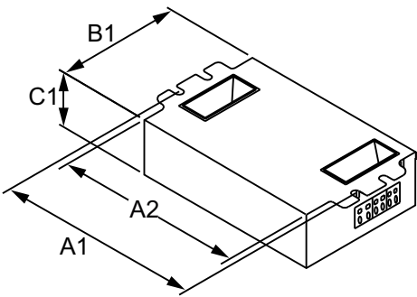
ELE DIM BAL (2) 26W CFL (4-PIN) 120-277V
