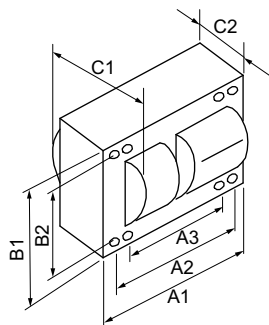
HPS BAL 1000W S52 5-TAP KIT WITH LAMP
