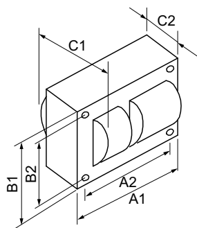
MH BAL 1000W M47 QUAD C&C
