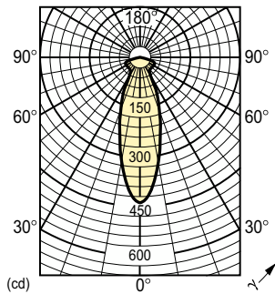
Light Distribution Diagram - Ref. 40W E14 240V NR50 30D FR 2BC/10
