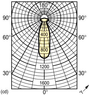
Light Distribution Diagram - REF SPOT 60W E27 240V NR63 30DFR2CT/4X3F
