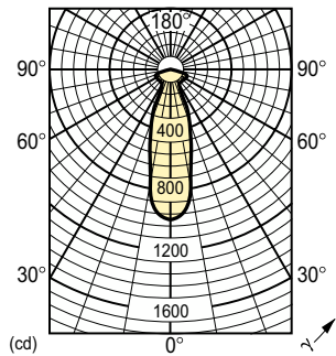
Light Distribution Diagram - Refl 60W E27 240V NR63 30D FR 1CT/6X5F
